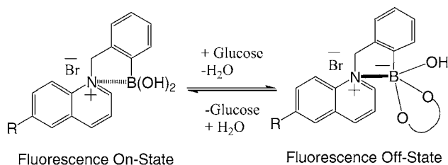
Fig. 4. A schematic representation of the charge neutralization–stabilization mechanism with regard to glucose sensing. The fluorescence off-state depicts the glucose-bound probe form. It should be noted that the figure reflects the increased B–N charge interaction in the presence of glucose, and not covalent bond formation.
